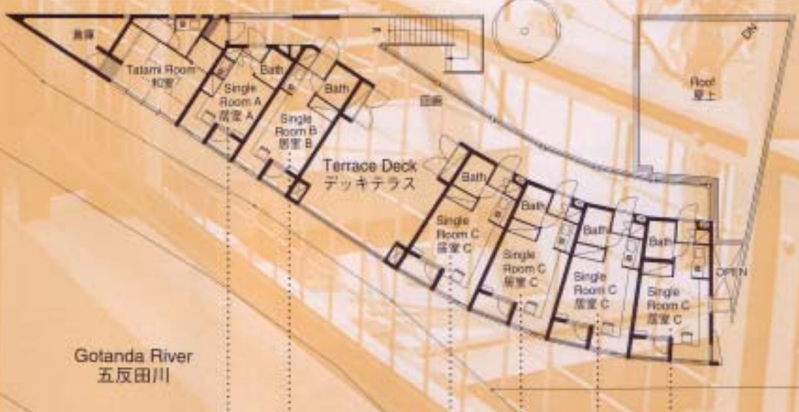
2F PLAN
