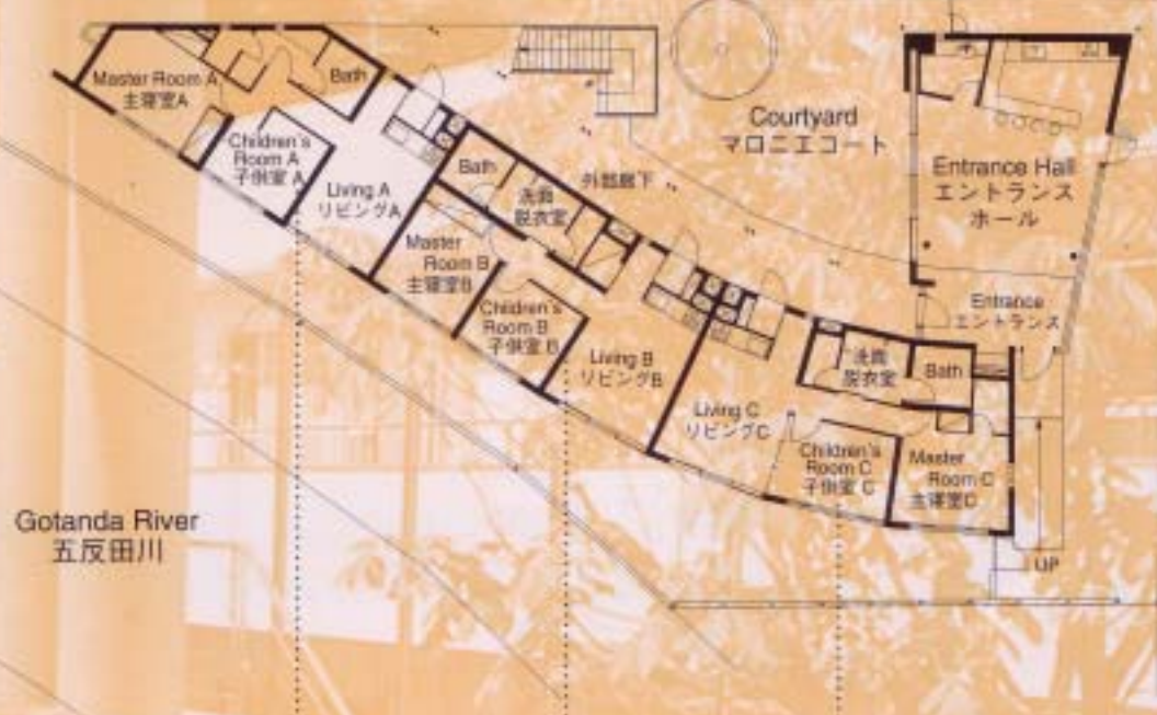
1F PLAN
